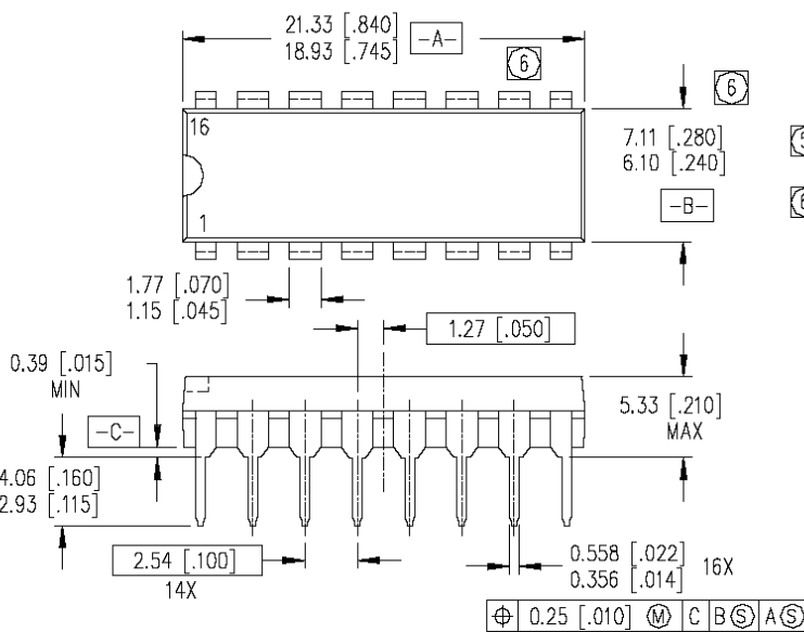
16-Lead PDIP
