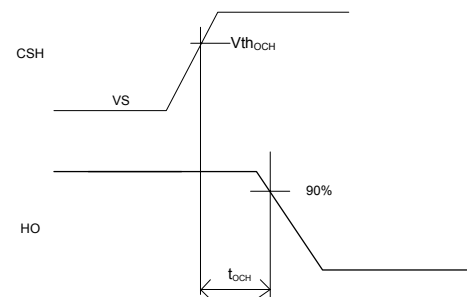
Figure 4. V_{CSH} > V_{TH,OCH} to Shutdown Waveform Definitions
