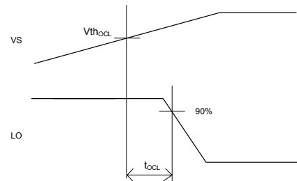
Figure 3. V_s > V_{TH,OCL} to Shutdown Waveform Definitions
