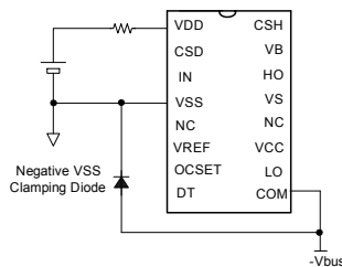
Figure 21. Negative V SS Clamping
